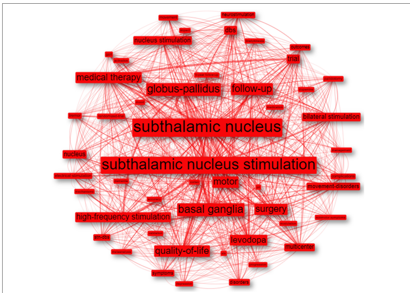
Figure 8. The conceptual structure according to KeyWords Plus™.
