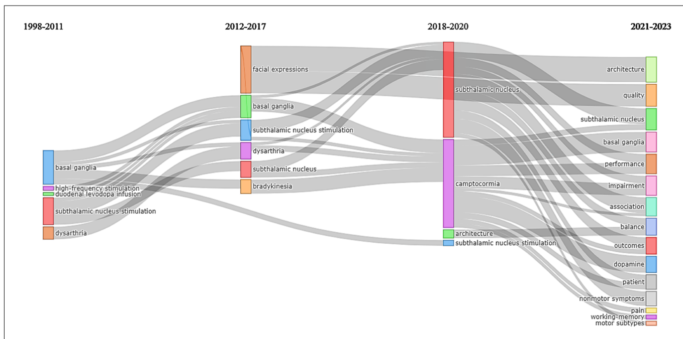
Figure 9. Thematic evolution according to KeyWords Plus™.
